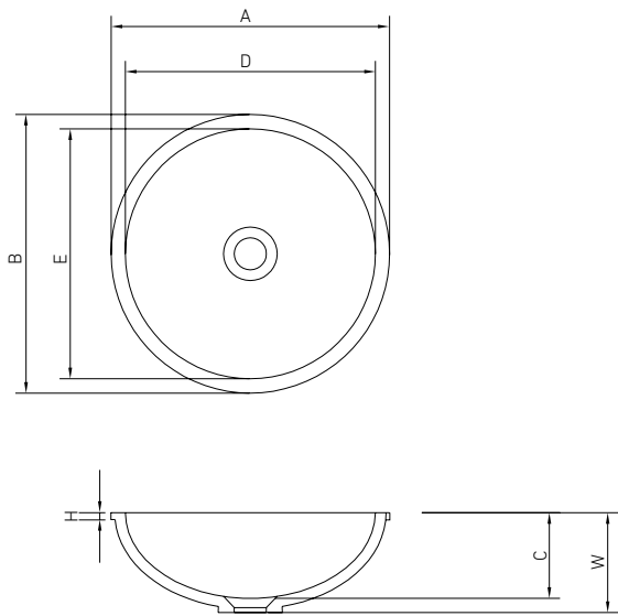
VAYER PURE 035.035.012.3-5.0.2.0 B Inset washbasin ø350
